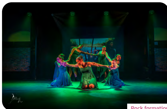
Rock formation
